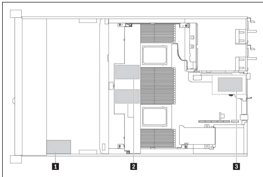
Figure 14. Potential locations of all supercaps in the SR630 V3 (2.5-inch drive configuration and standard heatsinks)
