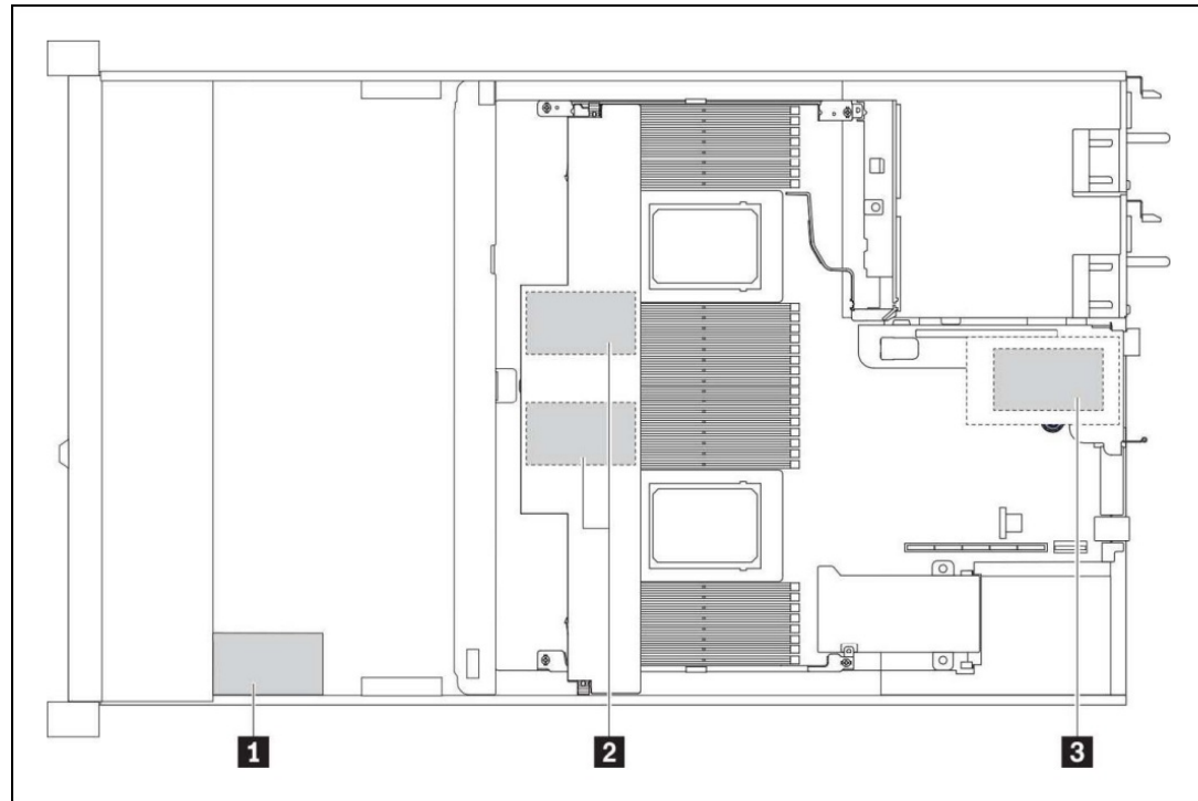
Figure 11. Location of the supercaps in the SR630 V3
