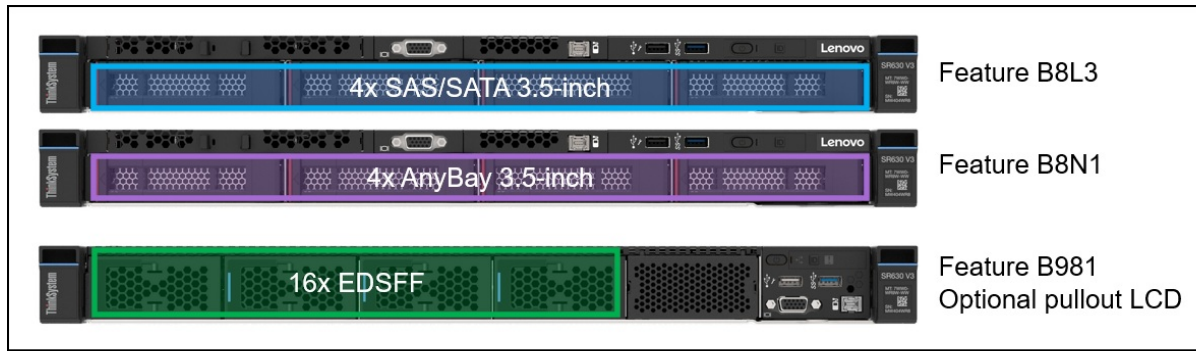
Figure 8. SR630 V3 front drive bay configurations - 3.5-inch and EDSFF drive bays
