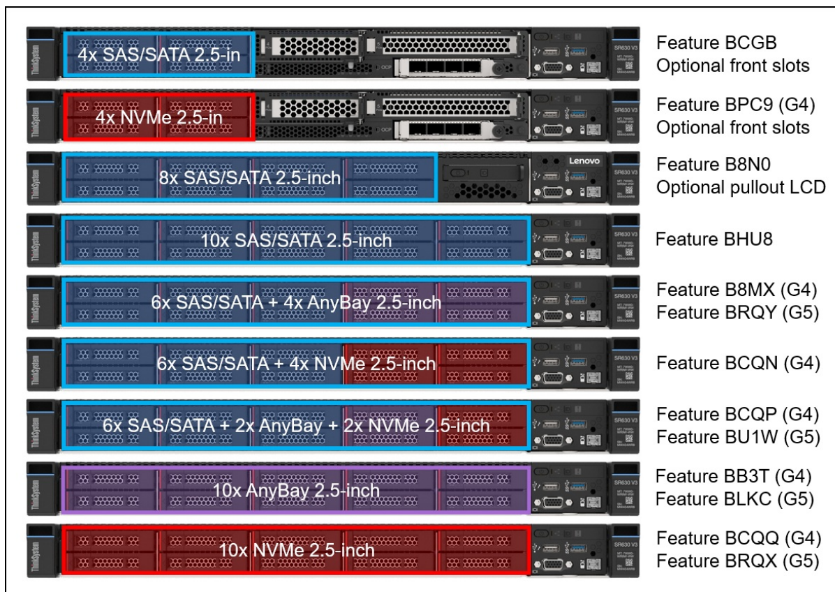
Figure 9. SR630 V3 front drive bay configurations - 2.5-inch drive bays
