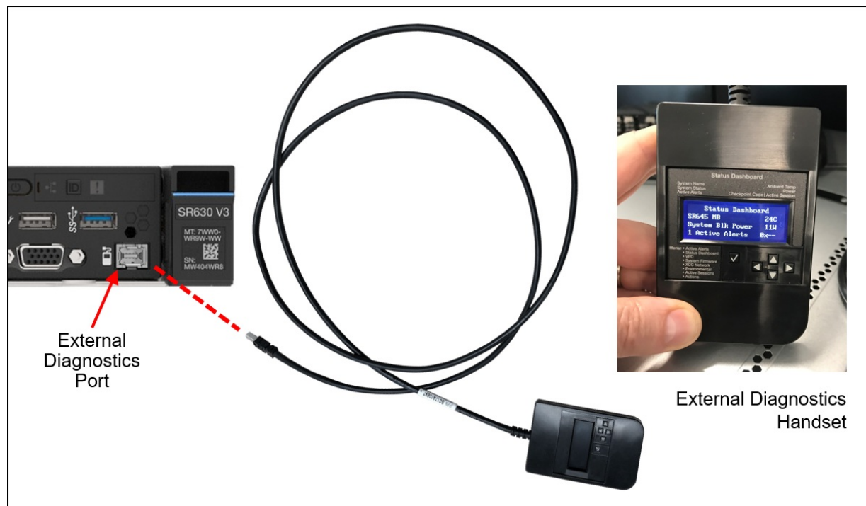
Figure 19. SR630 V3 External Diagnostics Handset
