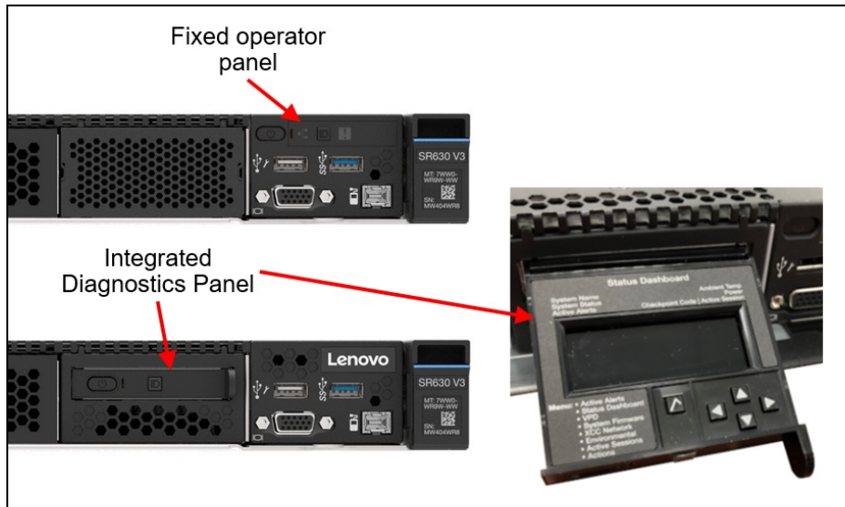
Figure 18. Operator panel choices for the 8x 2.5-inch drive bay configuration
