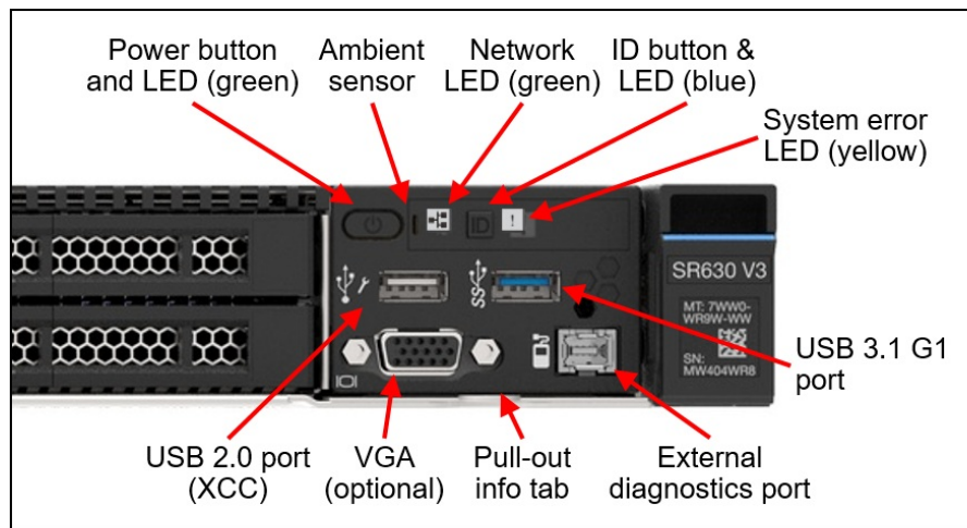
Figure 17. SR630 V3 Front operator panel
