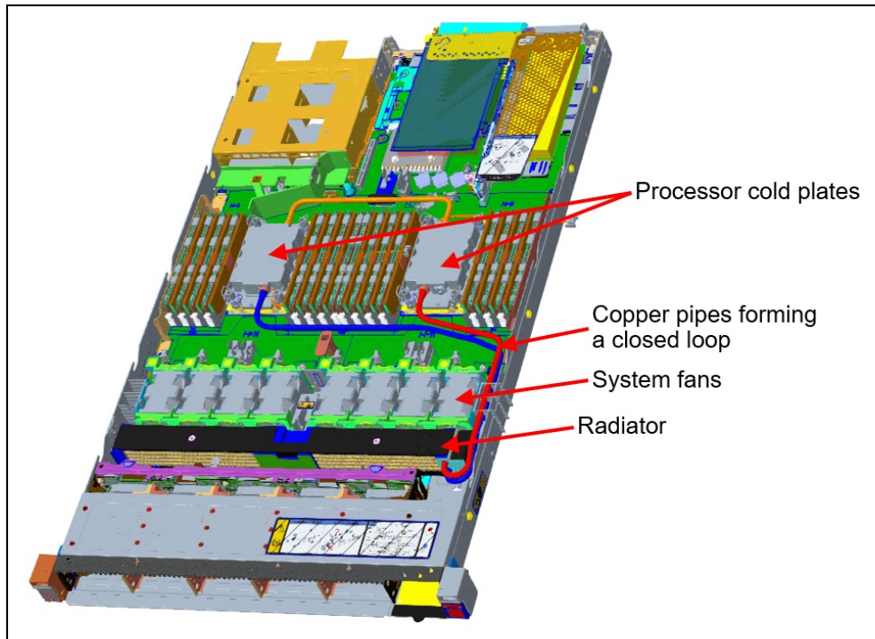
Figure 7. SR630 V3 with closed water loop (feature BRLJ)
