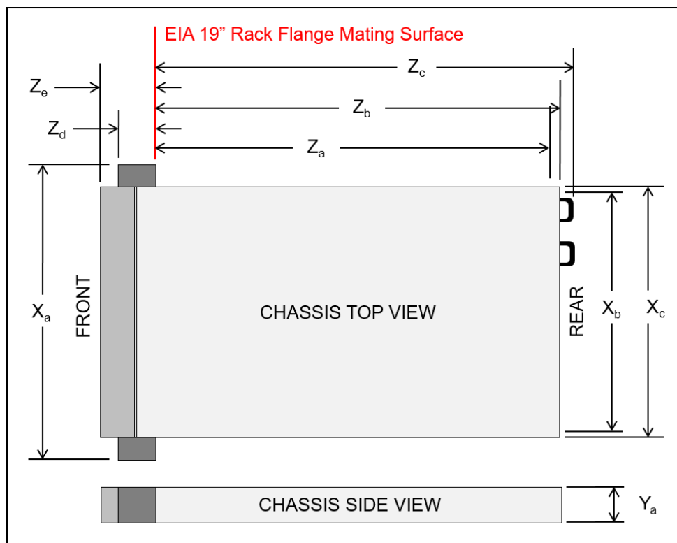
Figure 22. Server dimensions
